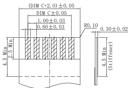
RECOMMENDED FFC/FPC
