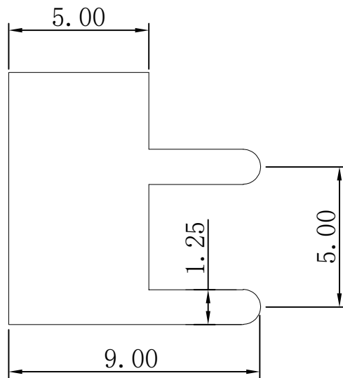
PCB LAYOUT
